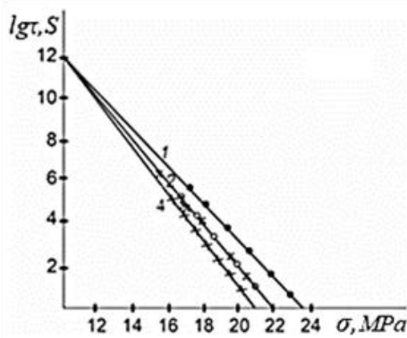
Fig.3. Stress dependence of the mechanical durability of HPPE film (initial) and its modifications: 1 - HPPE + 0.05 mass % CNT, 2 - HPPE (initial), 3 - HPPE + 0.03 mass % CNT, 4 - HPPE + 0.1 mass % CNT.
