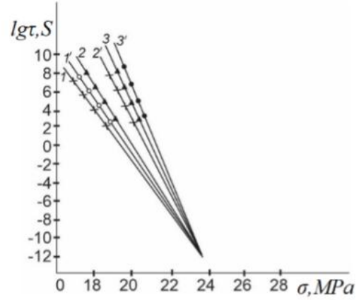
Fig.4. Strength dependence of the durability of HPPE film (1-3) and its optimal modification (1'-3') at different temperatures. 1, 2' - 173 K; 2 - 153 K; 3, 3' - 138 K; 1' - 223 K
