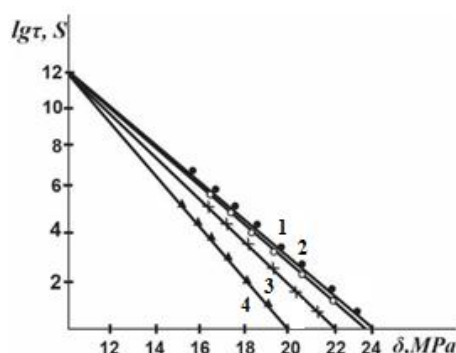
Fig. 5. Strength dependencies of the mechanical durability of the HPPE film and its modification before and after UV radiation in air: 1,2 - HPPE + 0.05 mass % CNT before and after UV radiation; 3,4 - HPPE (original) before and after UV radiation, t_{ob}=15 hours.
