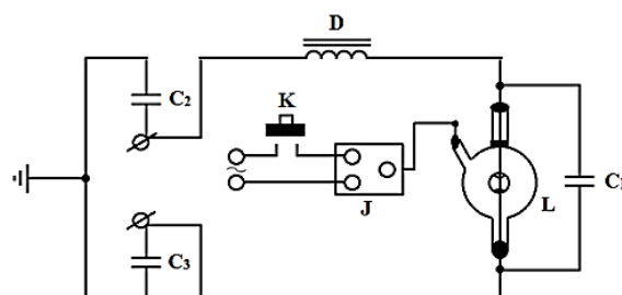
Fig. 1. Ignition block for the DRSH-500 lamp: D – ballast; L – lamp; K – end switch; J – ignition inductor with spark length of 15-20 mm; C1 – capacitor for shunting the lamp with a capacitance of 0.05 µF, rated for at least 250V; C2, C3 – capacitors with capacitance of 0.5 µF for grounding the network, with a rated voltage of at least 250V. Calibration of the effective UV radiation is attempted every 300 hours.
